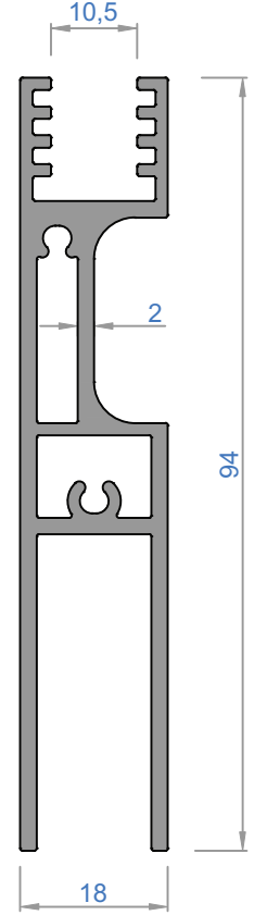
4452 - 1,368 kg/m
