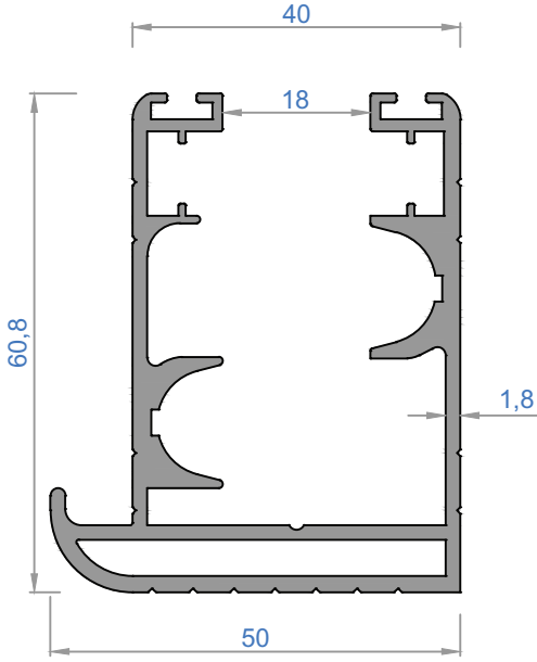
5787 - 1,540 kg/m
